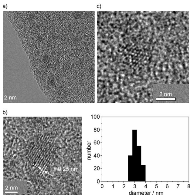
Figure 2. a) HRTEM image of rhodium nanocrystals supported on amorphous carbon film. The image shows that the nanocrystals do not agglomerate. b) HRTEM image (left) of a single 3-nm rhodium nanocrystal and particle size distribution (right) of the clusters: (3.1 \pm 0.4) nm. The measured distances between the crystallographic planes are in accord with the Rh–Rh distances reported for rhodium metal. c) HRTEM image of a rhodium nanocrystal oriented in the [111] direction. In this case as well, the measured distances between contrast maxima and minima can be interpreted in terms of the structural data of metallic rhodium.
