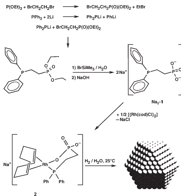
Scheme 1. Outline of the route that leads to phosphinophosphonic acid-stabilized rhodium clusters (represented, in this case, as a five-shell "magic number" cluster consisting of 561 rhodium atoms).
