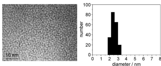
Figure 3. TEM image (left) of rhodium nanocrystals (2.5 nm) supported on amorphous carbon film and particle size distribution (right) of the clusters: (2.5 \pm 0.4) nm.
