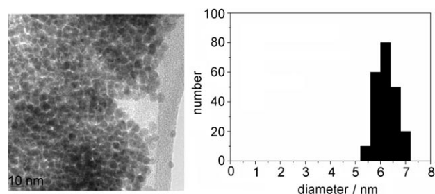
Figure 1. TEM image (left) of rhodium nanocrystals (6 nm) supported on amorphous carbon film and particle size distribution (right) of the clusters: (6.2 \pm 0.4) nm.
